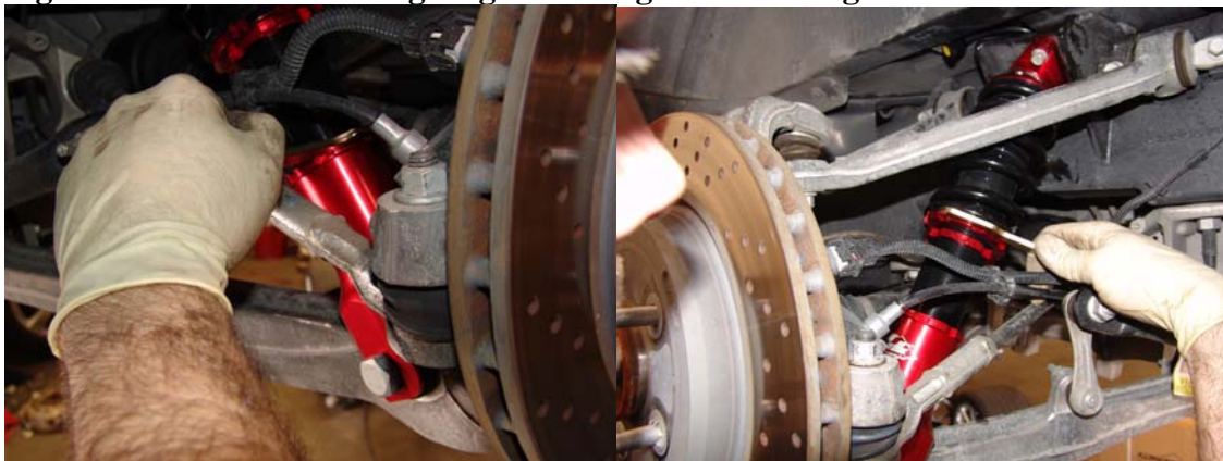
Figure 15a and 15b: Setting heights and tighten lock rings.
