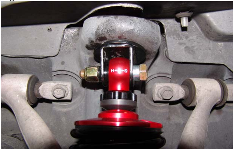
Figure 10 : Installation of front coil over
